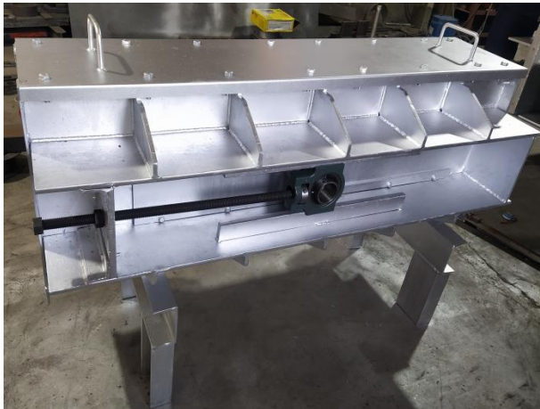
Fig.2g) Segment Frame
